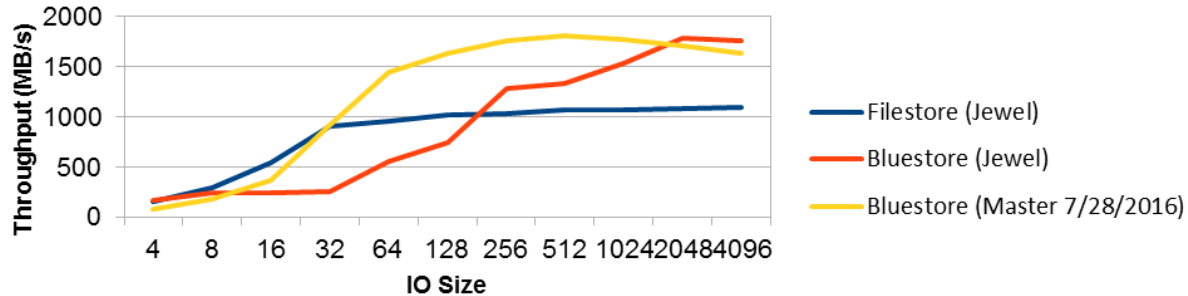
BlueStore vs FileStore NVMe Random RW Throughput
