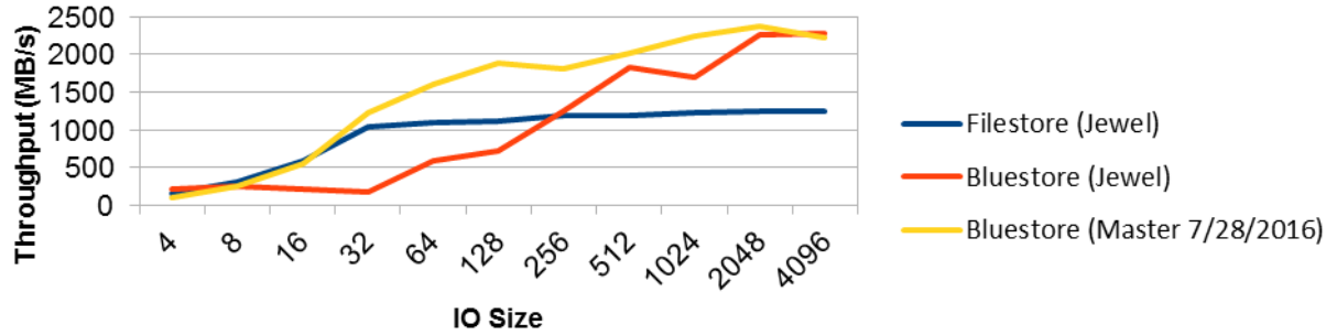
BlueStore vs FileStore NVMe Random Write Throughput
