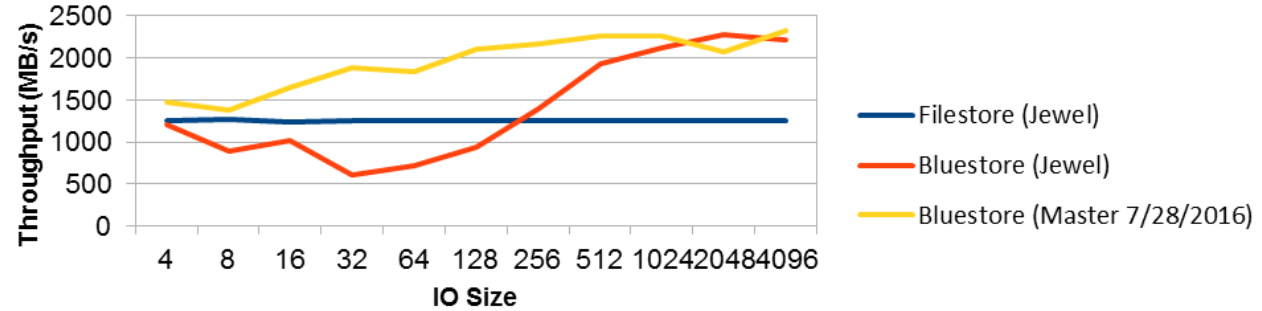
BlueStore vs FileStore NVMe Sequential Write Throughput
