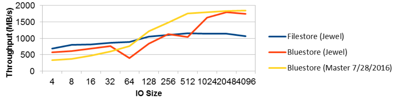
BlueStore vs FileStore NVMe Sequential RW Throughput
